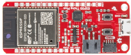
Sparkfun™ Thing Plus boards
