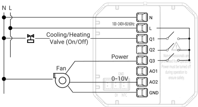
2-pipe, 2-Wire On/Off Valve, EC Fan
