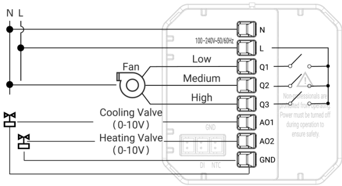
4-pipe, 0-10V Valve, 3 Speed Fan
