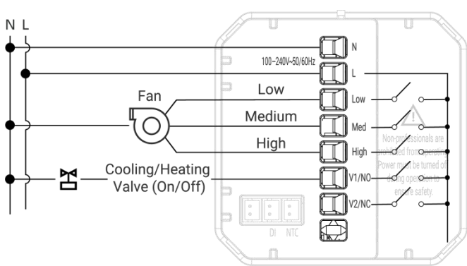
2-pipe, 2-Wire On/Off Valve, 3 Speed Fan
